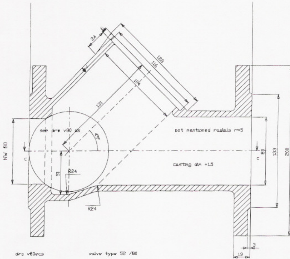
MONTI VALVES TYPE 52 NW 80
