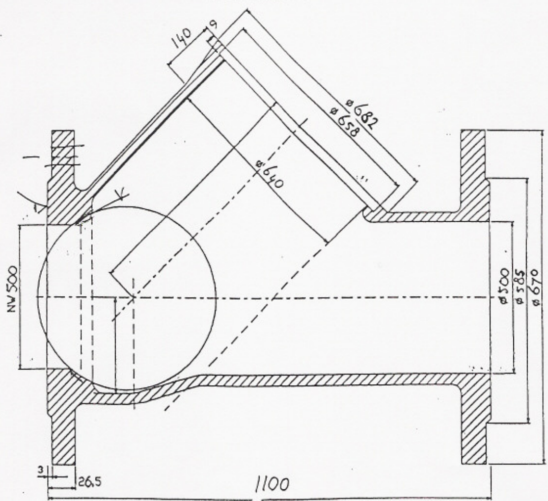
MONTI VALVES TYPE 52 NW 500
