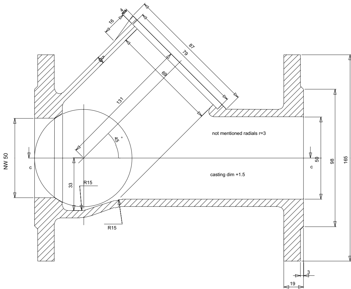
MONTI VALVES TYPE 52 NW 50
