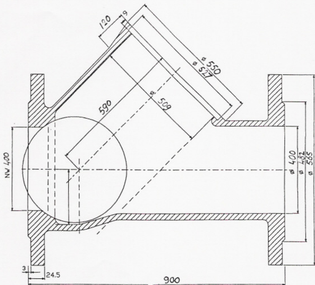
MONTI VALVES TYPE 52 NW 400
