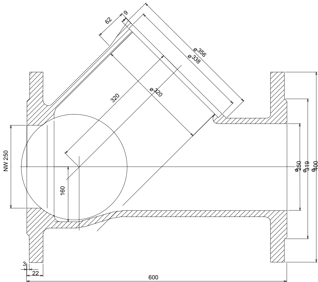
MONTI VALVES TYPE 52 NW 250
