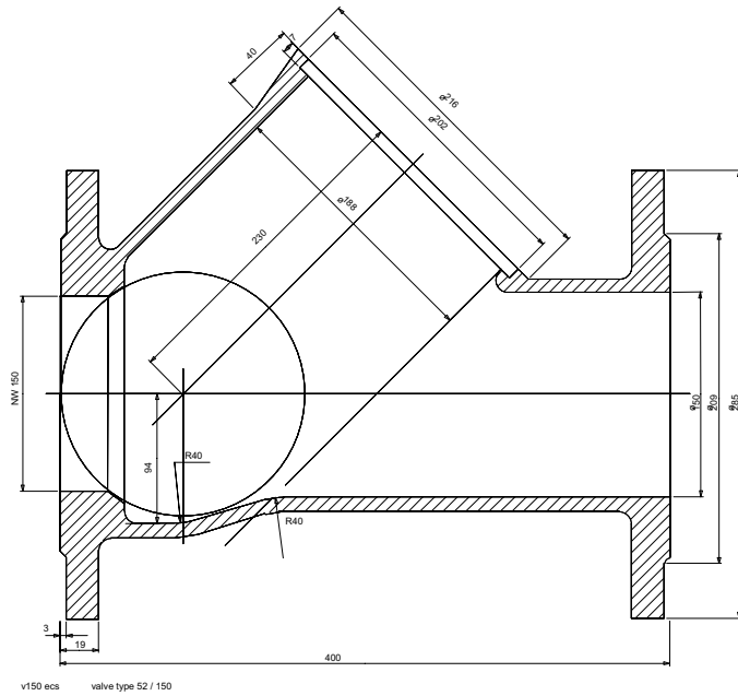
MONTI VALVES TYPE 52 NW 150
